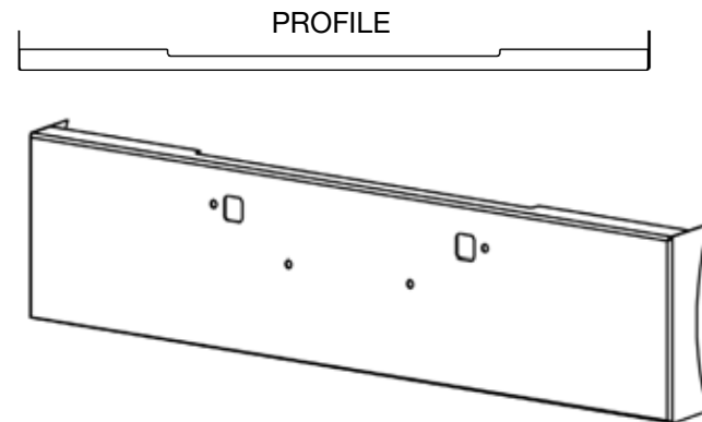
FRONT BUMPER BOX END WITH SIDE RADIUS
